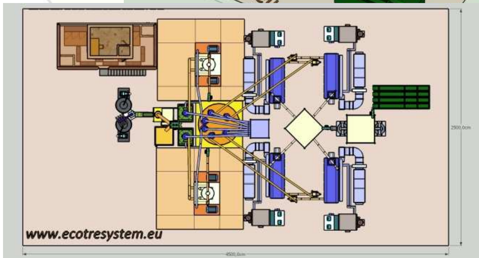
Plant 10t per hour
